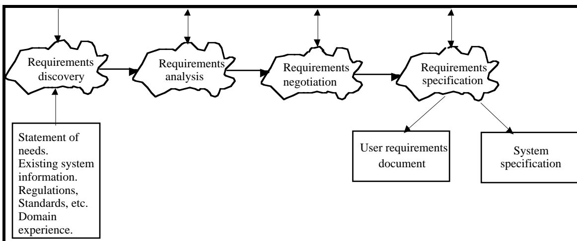
e 1 The requirements engineering process
