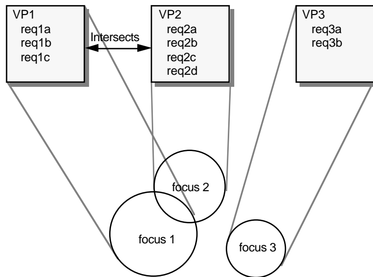
Figure 7 Viewpoints with overlapping and non-overlapping foci
